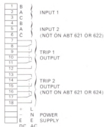
TERMINAL DIAGRAM
