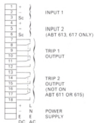
TERMINAL DIAGRAM
