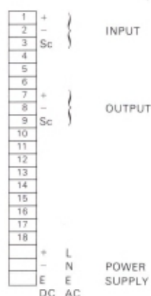
TERMINAL DIAGRAM ABM 740 AND 780
